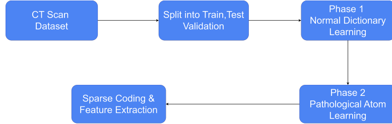
Figure 3.2: Model Training Workflow
